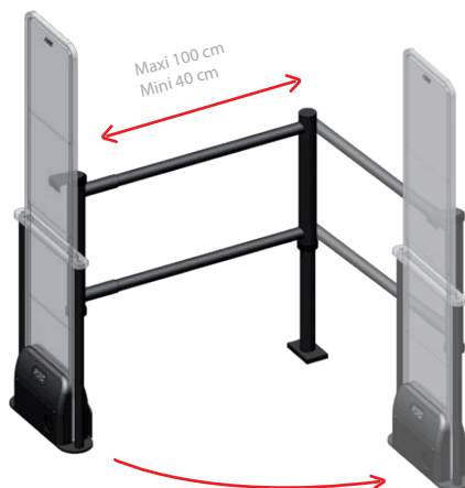
B ARM-PIVOT Rotation system
